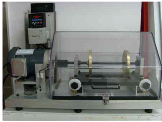
Rotor Kit (Machinery Fault Simulator)
